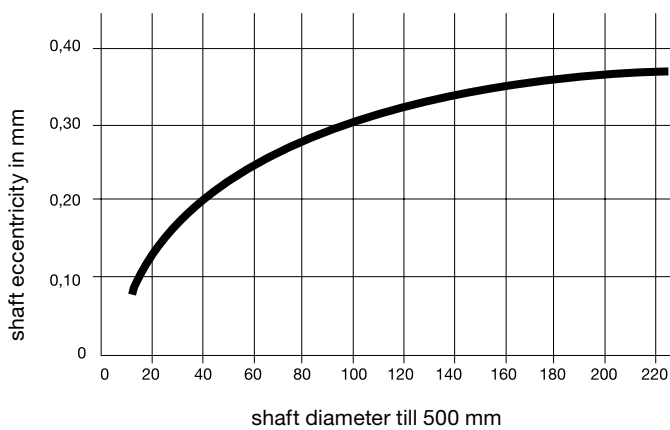
Above diagram shows the maximum allowable excentricity
